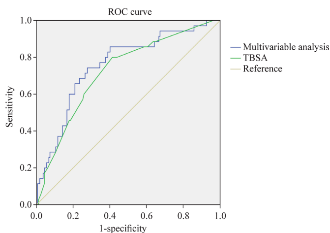
Figure 1 Receiver operating characteristic (ROC) curves based on risk factors and respective area under the ROC curves (AUCs). The blue ROC curve was based on all the potential risk factors used in multivariable logistic regression with model, whereas the green curve was computed using total burn surface area (TBSA) as the only factor.
